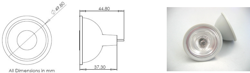
All Dimensions in mm
